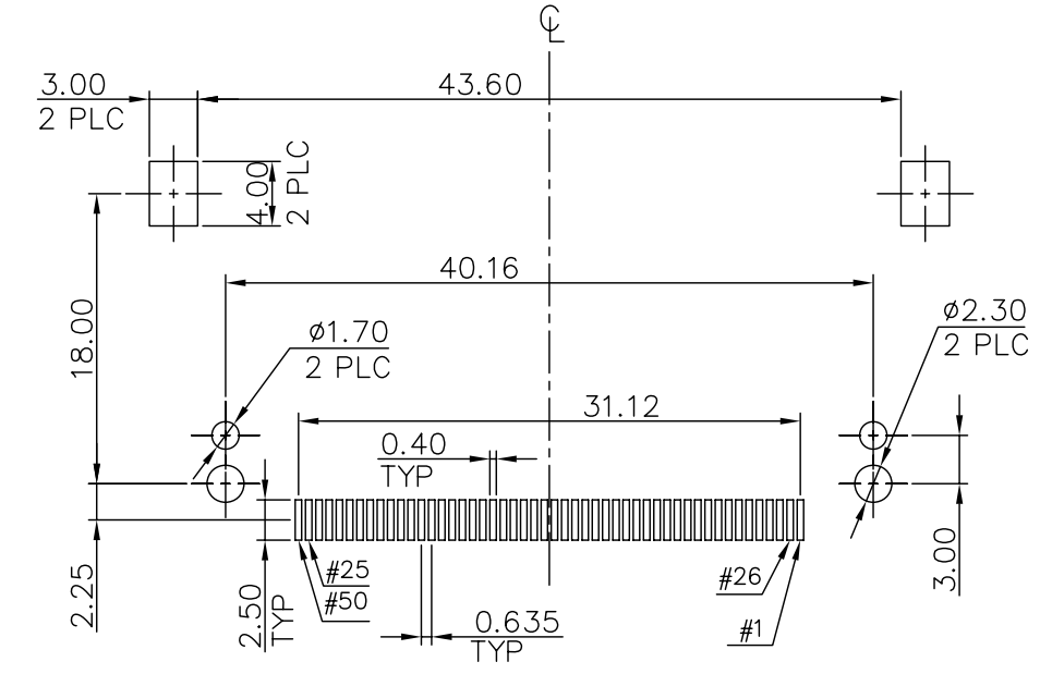
RECOMMENDED PCB LAYOUT (TOLERANCE: ±0.05)
